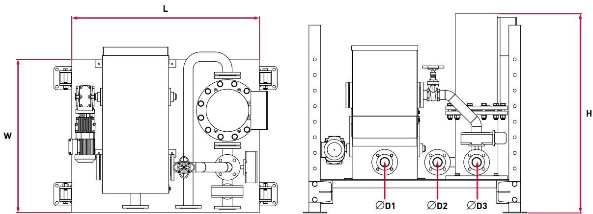
Diagram shows inline unit without integral pump
